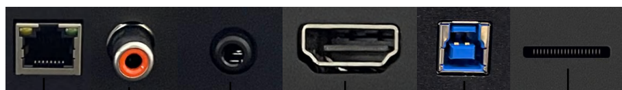
RJ45 SPDIF OUT EARPHONE (3.5mm AUDIO OUT) HDMI IN TOUCH USB TF Card
